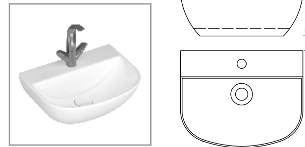
WALLHUNG BASIN CAT NO. SP7023 395 X 315 X 140 MM
