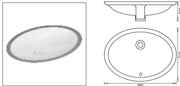
Small UNDER COUNTER BASIN CAT NO. SP7029 465 X 325 X 190 MM Big UNDER COUNTER BASIN CAT NO. SP7029 560 X 415 X 200 MM
