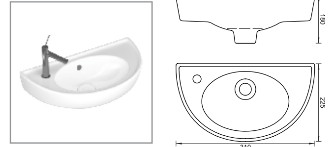
WALLHUNG BASIN CAT NO. SP6001 310 X 225 X 180 MM
