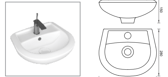
WALLHUNG BASIN CAT NO. SP6002 355 X 280 X 150 MM
