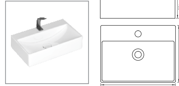
WALLHUNG BASIN CAT NO. SP7015 450 X 345 X 135 MM
