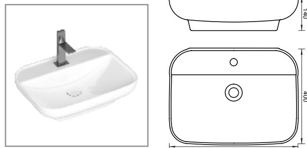
WALLHUNG BASIN CAT NO. SP7004 530 X 400 X 140 MM
